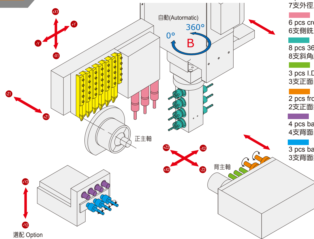
有導套之主軸構造 Using Live Bushing with Guide Bush
